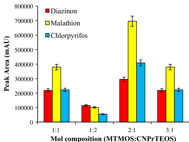
Fig. 1 Effect of different mol composition of the synthesized sol–gel hybrid MTMOS–CNPrTEOS on the extraction efficiencies of the three selected OPPs. Sol–gel parameters: \text{NH}_4\text{OH} pH 10.0 and 80 °C drying temperature
