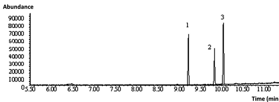
Fig. 6 GC Chromatogram of OPPs mixture from direct injection: 1 diazinon, 2 malathion and 3 chlorpyrifos with concentration of 100 \mu\text{g mL}^{-1} . GC conditions: HP-5 column ( 25 \text{ m} \times 0.20 \text{ mm i.d.} ,
