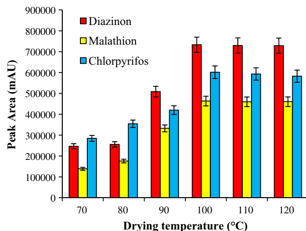
Fig. 3 Variation of extraction efficiency with drying temperature for three selected OPPs using sol–gel hybrid of mol composition 2:1 mol ratio MTMOS–CNPrTEOS as SPE sorbent. Sol–gel parameters: \text{NH}_4\text{OH} pH 10.5
