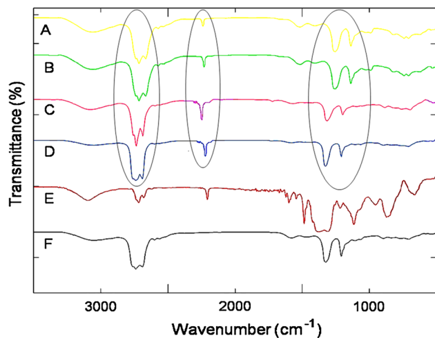
Fig. 4 Fourier transform infrared spectra of sol-gel hybrid with molar ratio of a 3:1 MTMOS:CNPrTEOS, b 2:1 MTMOS:CNPrTEOS, c 1:2 MTMOS:CNPrTEOS, d 1:1 MTMOS:CNPrTEOS, e raw CNPrTEOS and f raw MTMOS
