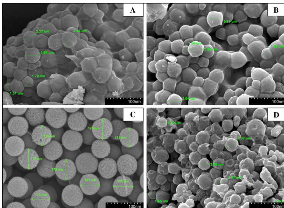
Fig. 5 SEM micrographs of sol-gel hybrid MTMOS-CNPrTEOS with mol composition of (a) 1:1 MTMOS:CNPrTEOS at \times 5 k magnification, (b) 1:2 MTMOS:CNPrTEOS at \times 5 k magnification,
