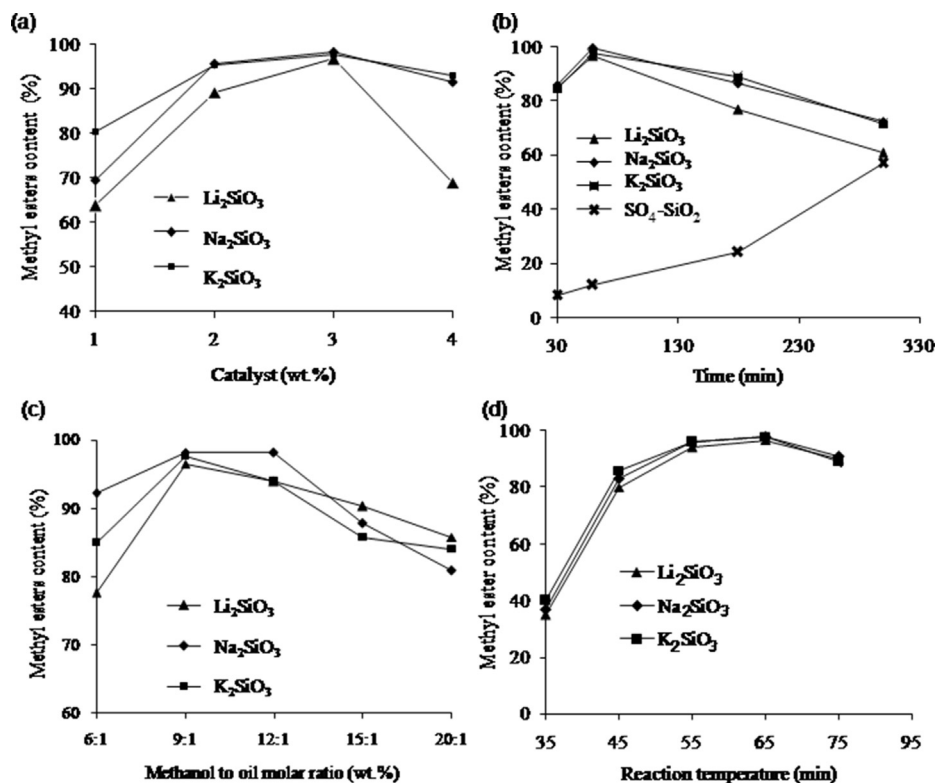
Fig. 5. Effect of (a) catalysts amount, (b) reaction duration, (c) methanol to oil molar ratio (d) reaction temperature in transesterification using alkali metals silicate as catalysts.
